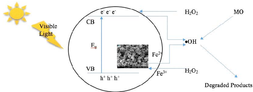
Figure 5. Diagram showing the mechanism of degradation of methyl orange using photo-fenton mechanism.
