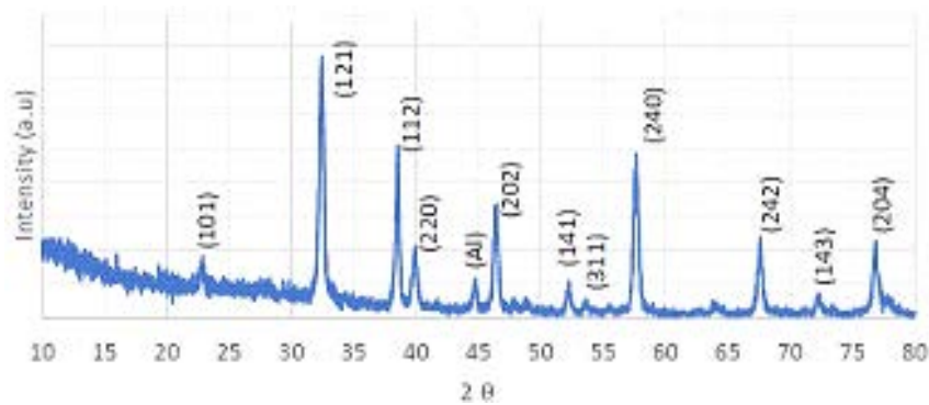
Figure 1. XRD graph of Lanthanum orthoferrite.
