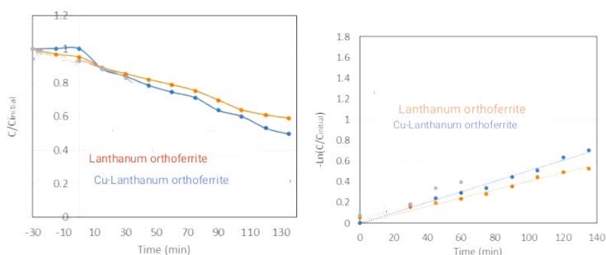
Figure 4. Photo degradation of methyl orange using Lanthanum orthoferrite doped with Copper. (The pseudo-first-order kinetic was observed for Lanthanum orthoferrite and 15 Cu Lanthanum orthoferrite both of which have similar photo catalytic activity with a kinetic constant k value of approximately 0.003/min and R^2 value of 0.99. Lanthanum orthoferrite only displays with a R^2 value of 0.98 with the apparent k value of 0.0064/min.)
