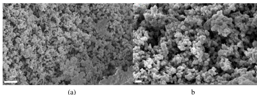
Figure 3. SEM images of: (a) Lanthanum orthoferrite; and (b) Cu doped Lanthanum orthoferrite.
