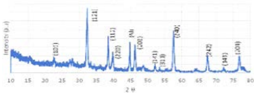
Figure 2. XRD graph of metal doped Lanthanum orthoferrite.
