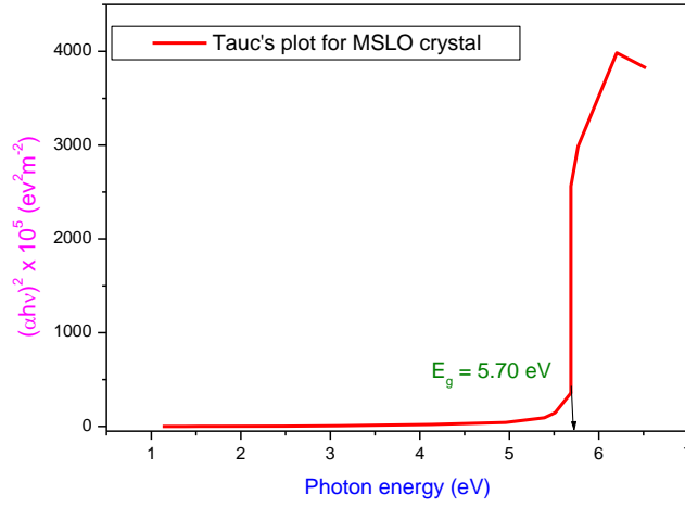
Figure 6. Tauc's plot for MSLO crystal.
