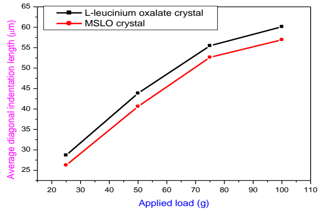
Figure 15. Plots of average diagonal indentation length versus applied load for undoped and magnesium sulfate-doped L-leucinium oxalate (MSLO) crystal.
