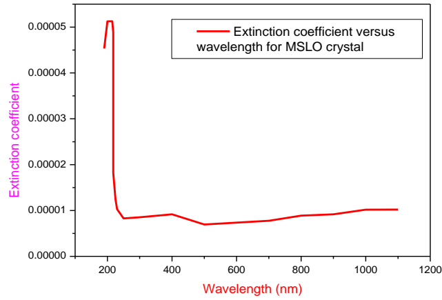
Figure 7. Plot of extinction coefficient versus wavelength for MSLO crystal.
