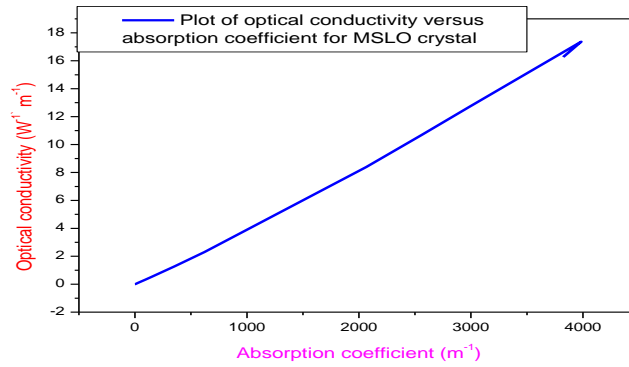
Figure 10. Plot of optical conductivity (in SI units) versus absorption coefficient for MSLO crystal.
