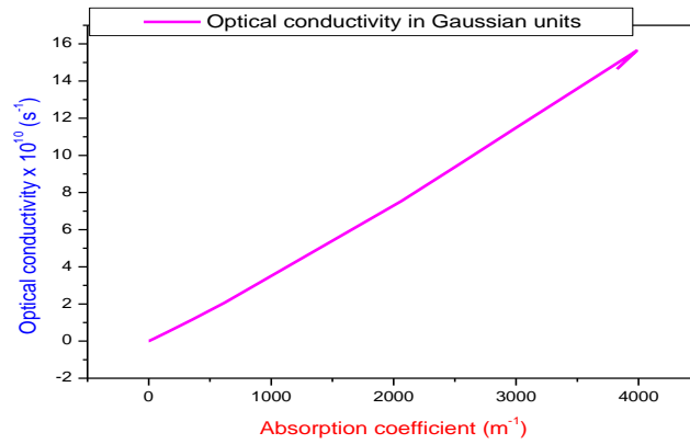
Figure 11. Plot of optical conductivity (in Gaussian units) versus absorption coefficient for MSLO crystal.
