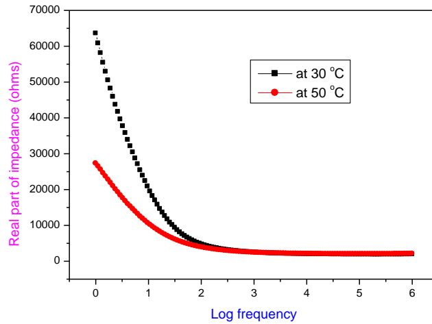
Figure 12. Real part of impedance variation with frequency at different Temperatures for MSLO crystal.
