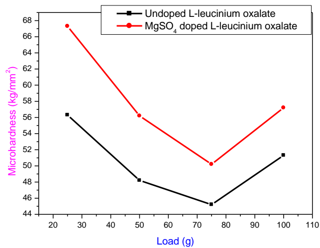
Figure 16. Plots of microhardness versus applied load for undoped and Magnesium sulfate-doped L-leucinium oxalate (MSLO) crystal.
