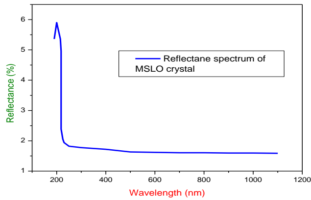
Figure 8. Reflectance spectrum of MSLO crystal.
