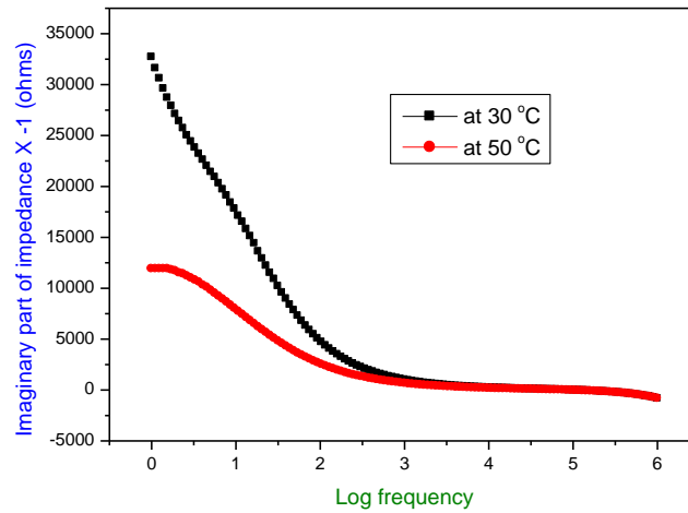
Figure 13. Imaginary part of impedance variation with frequency at different Temperatures for MSLO crystal.
