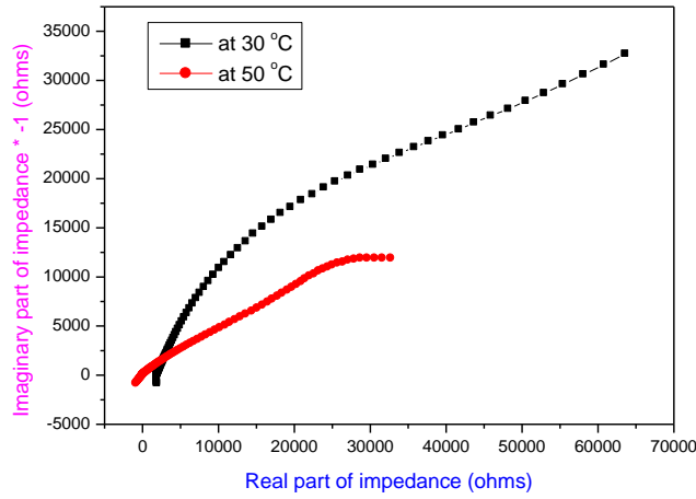
Figure 14. Nyquist plot of the grown MSLO crystal.
