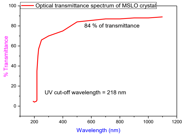
Figure 4. UV-Vis-NIR transmittance spectrum of MSLO crystal.
