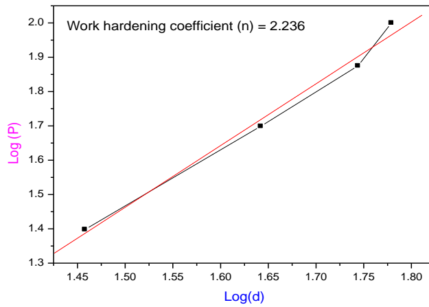
Figure 17. Plot of \log(P) versus \log(d) for undoped L-leucinium oxalate crystal.
