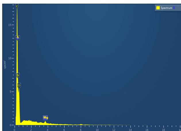
Figure 19. EDS spectrum of MSLO crystal.
