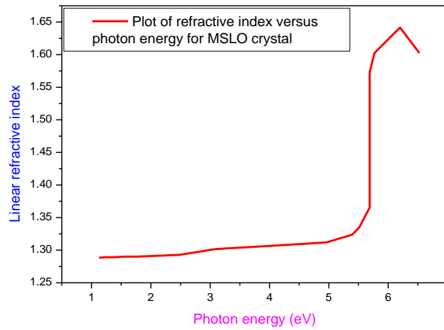
Figure 9. Variation of refractive index with photon energy for MSLO crystal.
