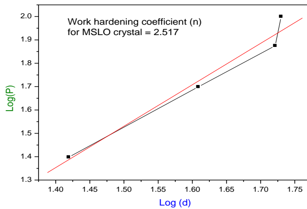
Figure 18. Plot of \log(P) versus \log(d) for MSLO crystal.
