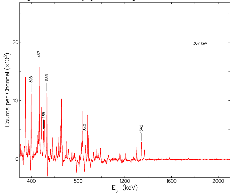
Figure 4. Gamma-ray spectrum with gate on 307-keV transition.
