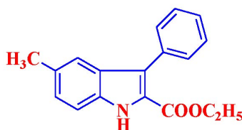
Figure 1. Structure of ethyl 5-methyl-3-phenyl-1H-indole-2-carboxylate (5-MPIC).
