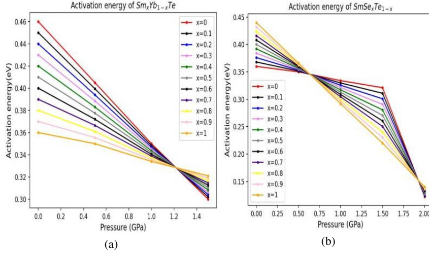
Figure 4. Variation of activation energy with pressure at given different concentration ( x ).
