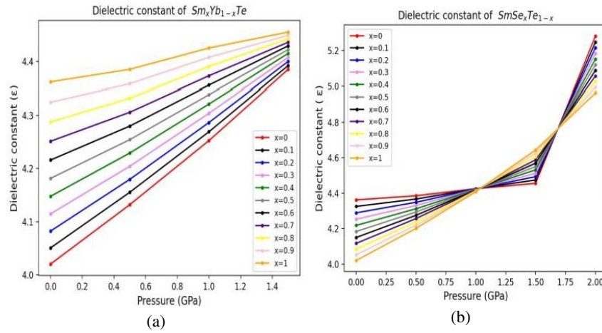
Figure 8. Variation of dielectric constant with pressure at given different concentration ( x ).
