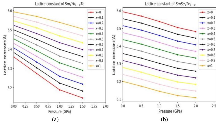
Figure 2. Variation of lattice constant with pressure at given different concentration ( x ).
