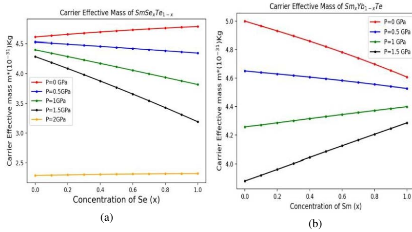
Figure 5. Variation of carrier effective mass with pressure at given different concentration ( x ).
