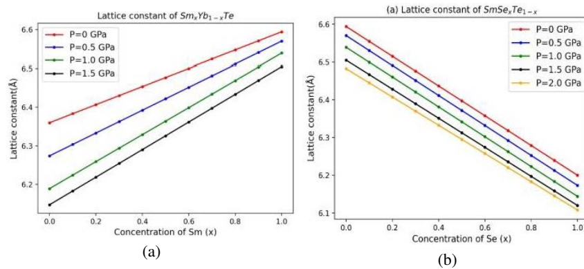
Figure 1. Variation of lattice constant with concentration ( x ) at given different pressure.
