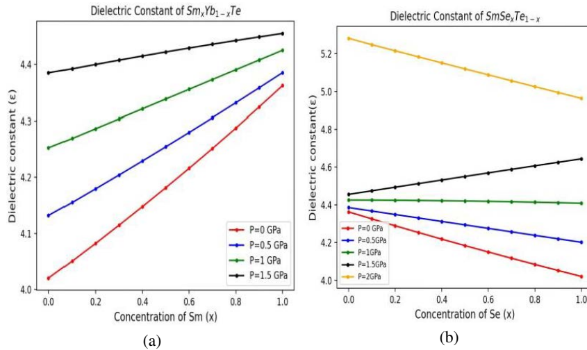
Figure 7. Variation of dielectric constant with concentration ( x ) at given different pressure.
