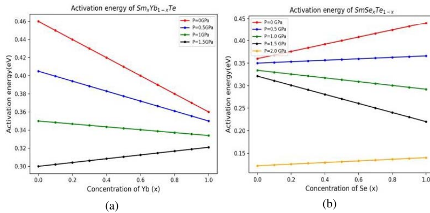
Figure 3. Variation of activation energy with concentration ( x ) at given different pressure.
