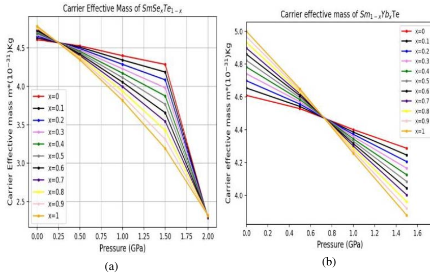
Figure 6. Variation of carrier effective mass with concentration ( x ) at given different pressure.
